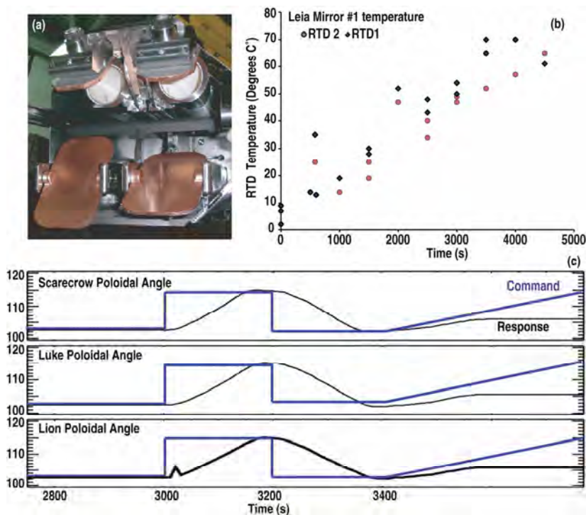
Fig. 4. ECH dual launcher photo (a), temperature of the focusing mirror (b), and response to a step command (c).
