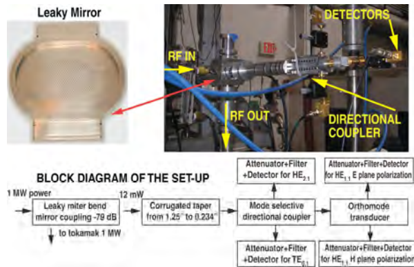
Fig. 7. Experimental setup for the four-port power divider.
