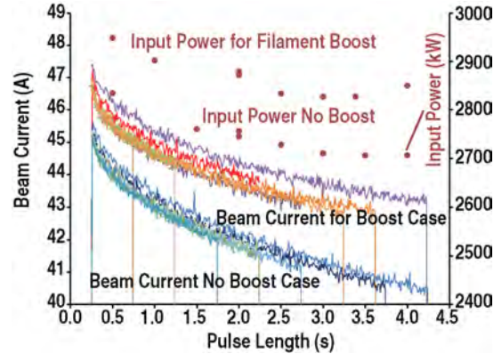
Fig. 2. Electron beam current with and without filament boost, and input power vs pulse length for the recently installed depressed collector gyrotron. The filament voltage is increased by 20% 6 s before the pulse for boosted pulses.
