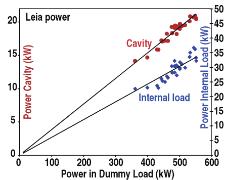
Fig. 5. Gyrotron cavity and internal load power loading versus the power measured in a dummy load at the tokamak.
