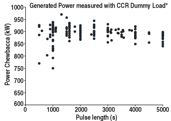
Fig. 3. Power measured vs pulse length measured during testing of the depressed collector gyrotron. *Calabazas Creek Research, Saratoga, CA.
