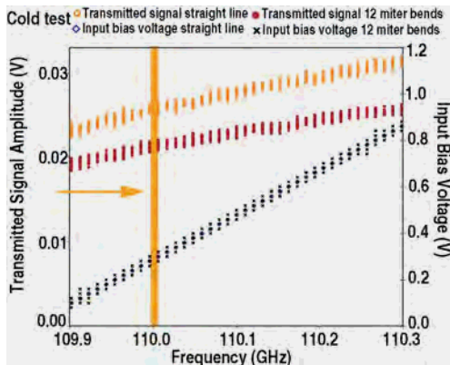
Fig. 6. Cold Test transmission efficiency results showing the transmitted amplitude for a straight waveguide in orange and for 12 miter bends in red, together with the biasing voltage in blue and black.
